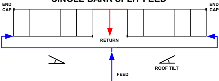
SINGLE BANK SPLIT FEED
