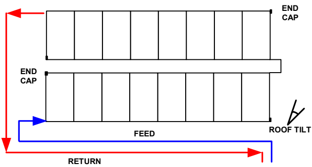
BANKS IN SERIES
