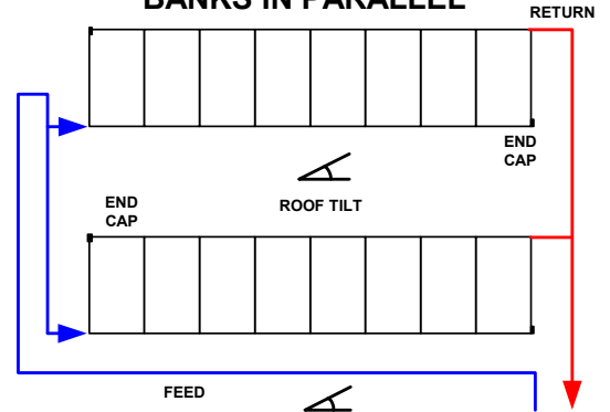
BANKS IN PARALLEL
