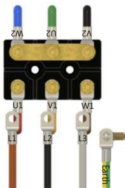
UPH400 WYE/STAR Connection
