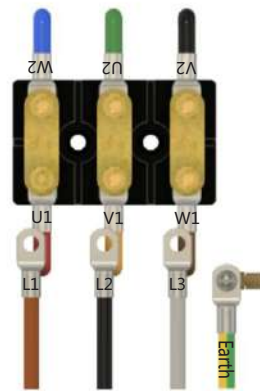
UPH550/UPH700 Delta Connection
