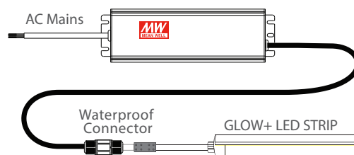
With 24V DC wiring diagram
