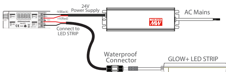
With Dimmer wiring diagram
