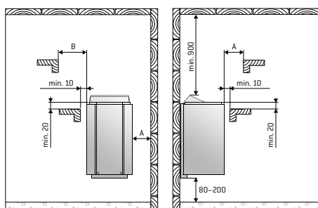
Vega Compact, safety distances (mm)
